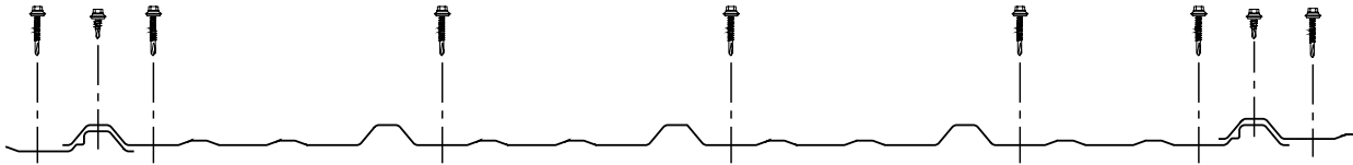
Pro-Panel II Fastening Pattern - Interior
