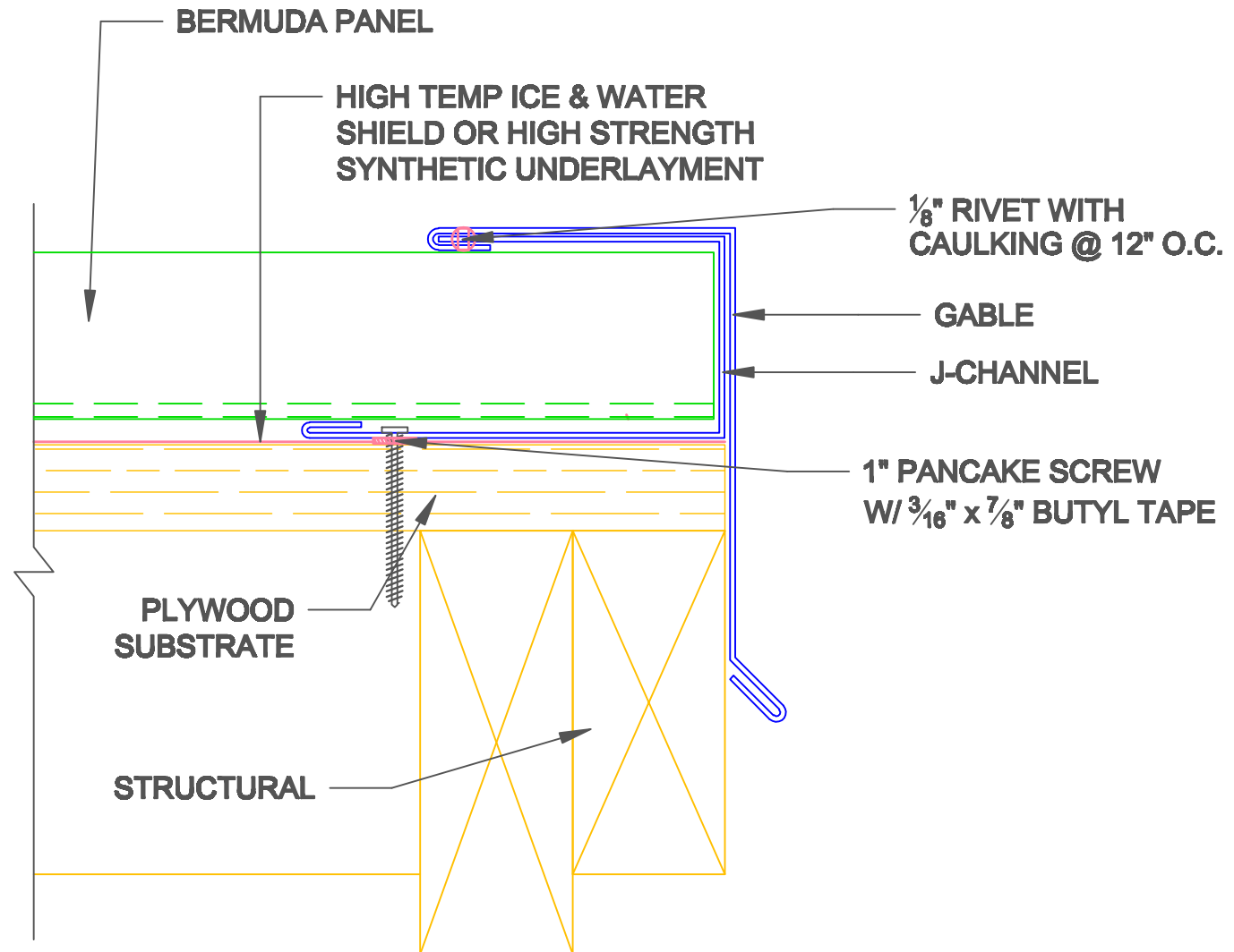
BERMUDA GABLE W/ J-CHANNEL
