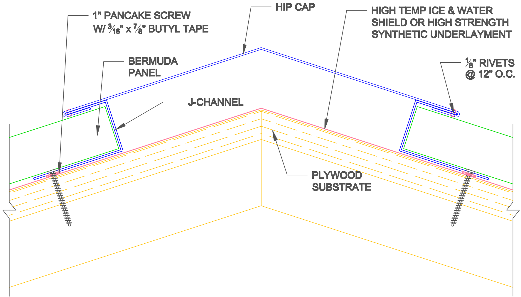
BERMUDA HIP W/ J-CHANNEL
