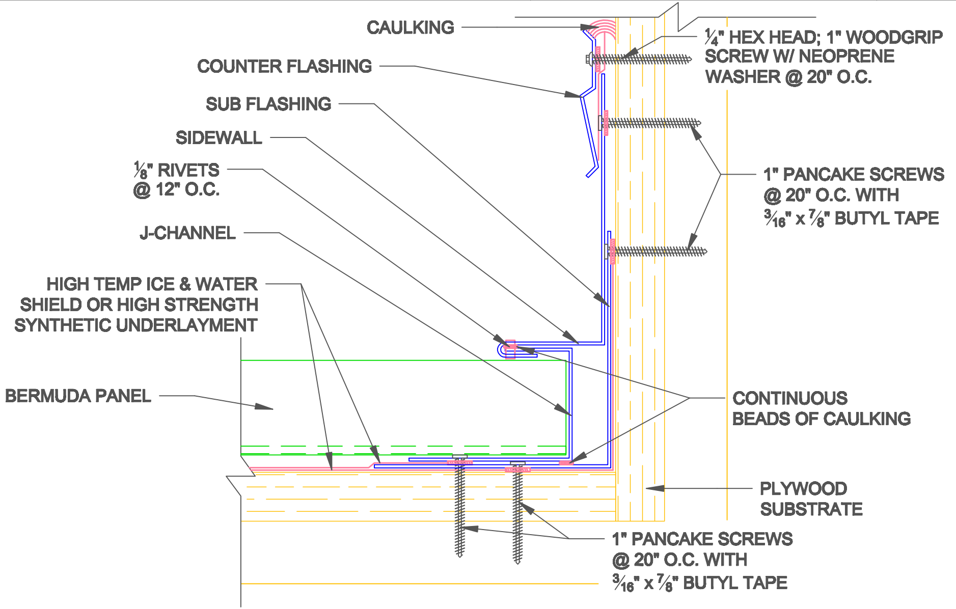
BERMUDA SIDEWALL W/ COUNTER FLASHING
